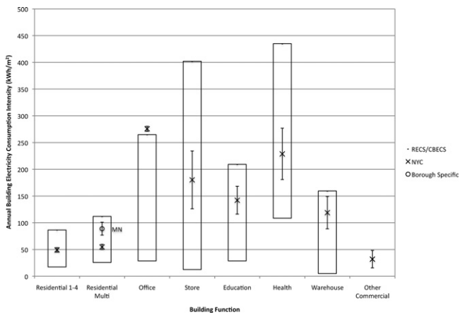
Fig. 3. Annual building electricity consumption intensity estimates by building function (kWh/m 2 ), 2009.
