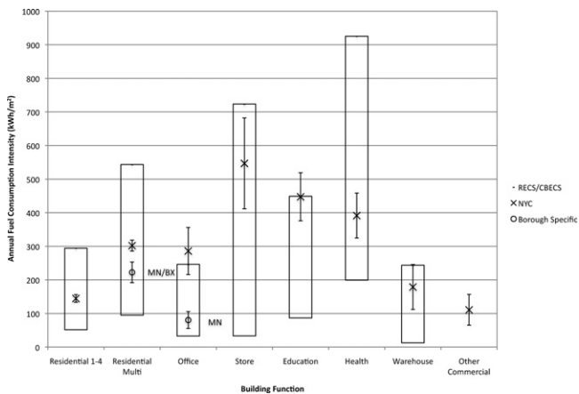
Fig. 4. Annual building total fuel consumption intensity estimates by building function (kWh/m 2 ), 2009.
