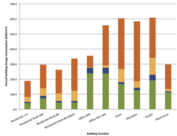
Fig. 5. Annual building energy consumption intensities by end use and building function (kWh/m 2 ), 2009.
